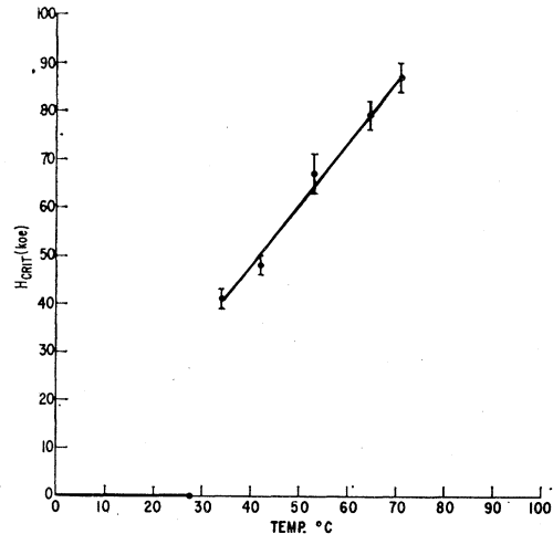
FIG. 12. The critical field vs the temperature as determined from Fig. 11. The critical field represented here is chosen as the onset of the increase in magnetic moment of the sample.
